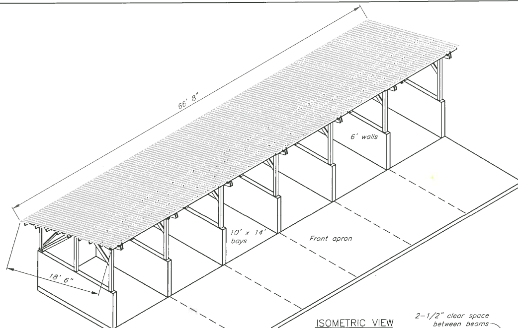
ISOMETRIC VIEW
