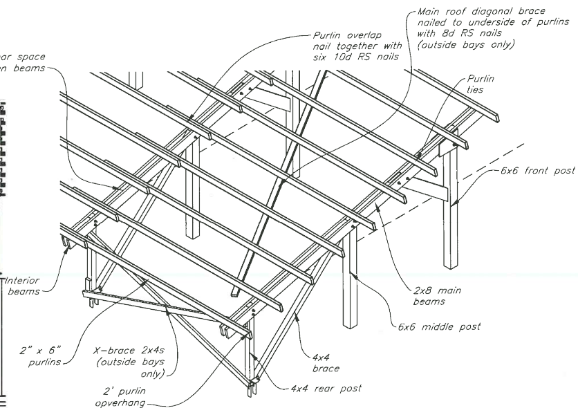
ISOMETRIC TIMBER DETAIL VIEW
