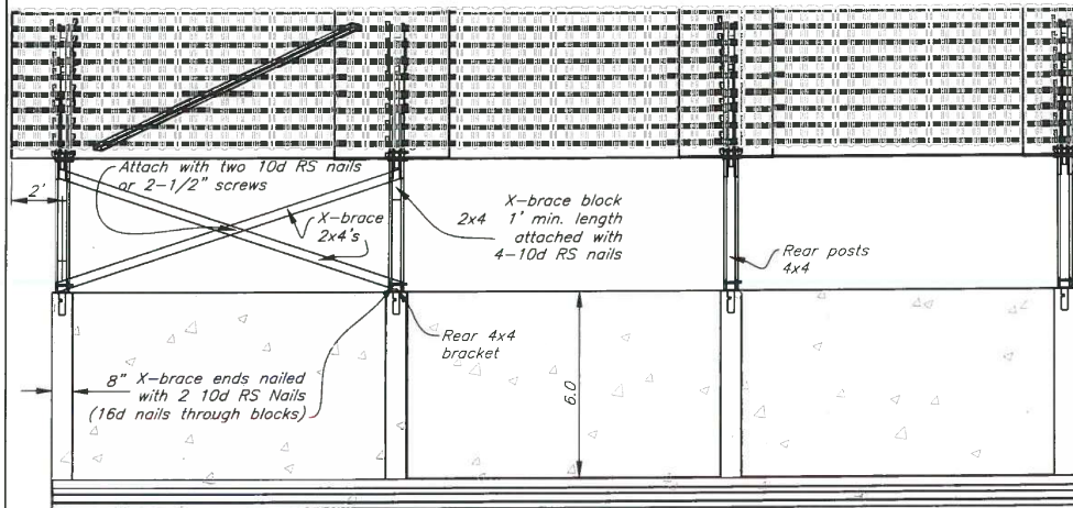
PARTIAL REAR ELEVATION
